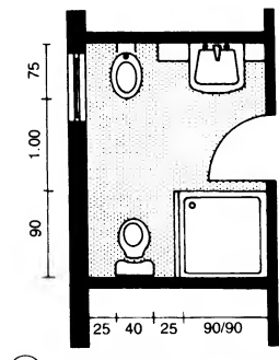
⑮ Shower, WC, bidet, basin
